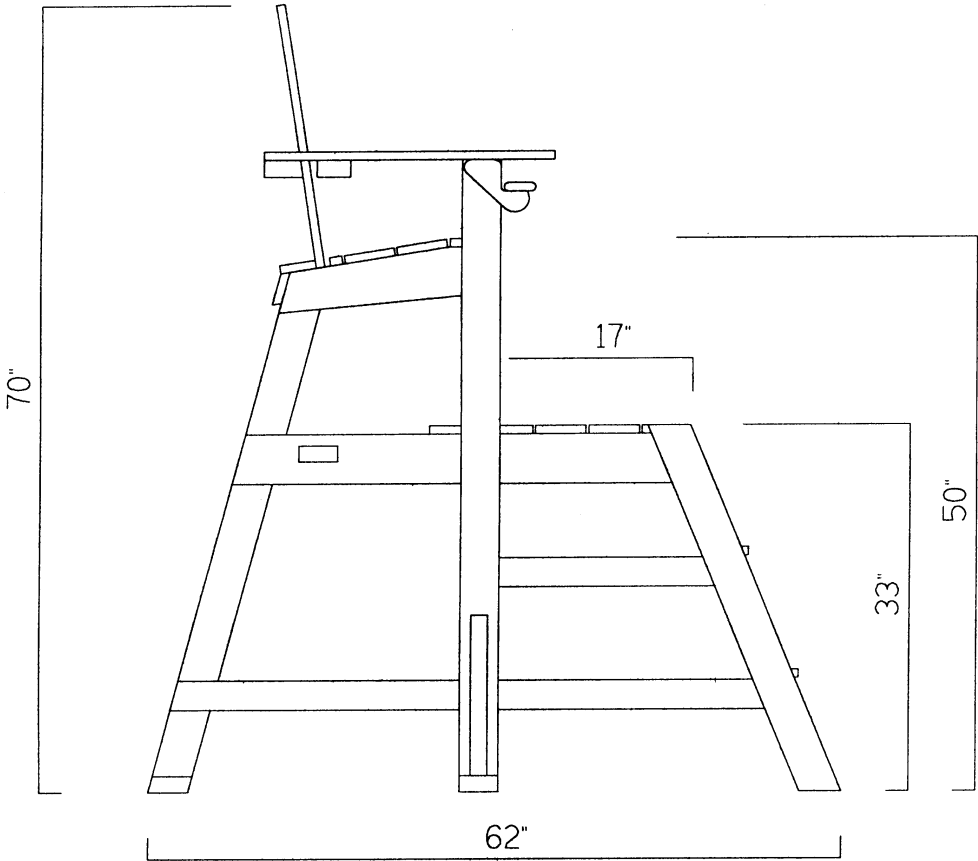
SIDE VIEW
